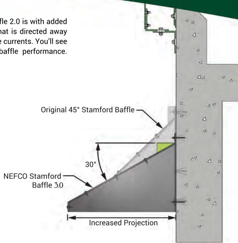
WALL MOUNTED BAFFLE
